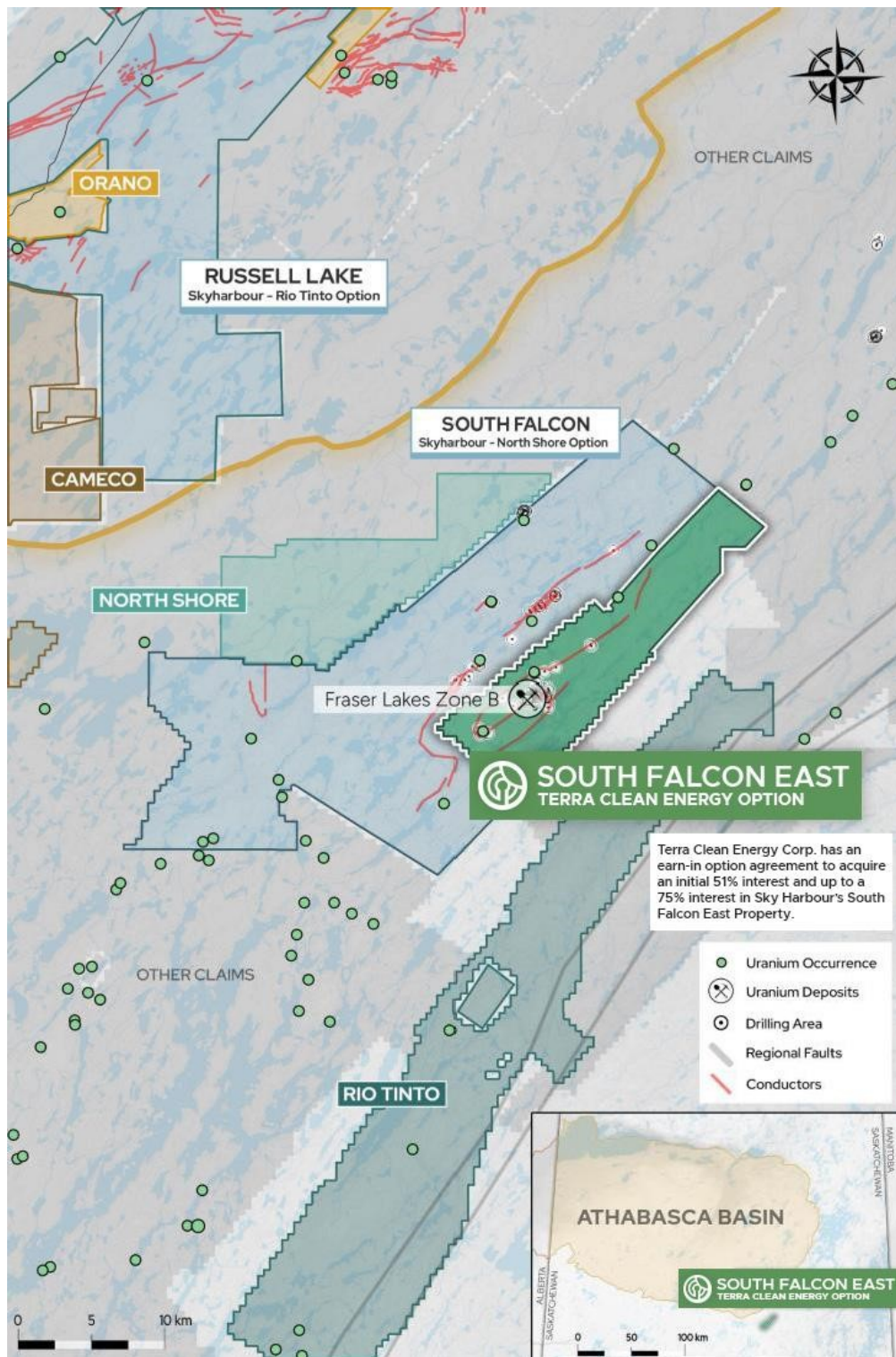
Figure 2: Fraser Lakes B Uranium Deposit, South Falcon East project, Saskatchewan About English River First Nation
